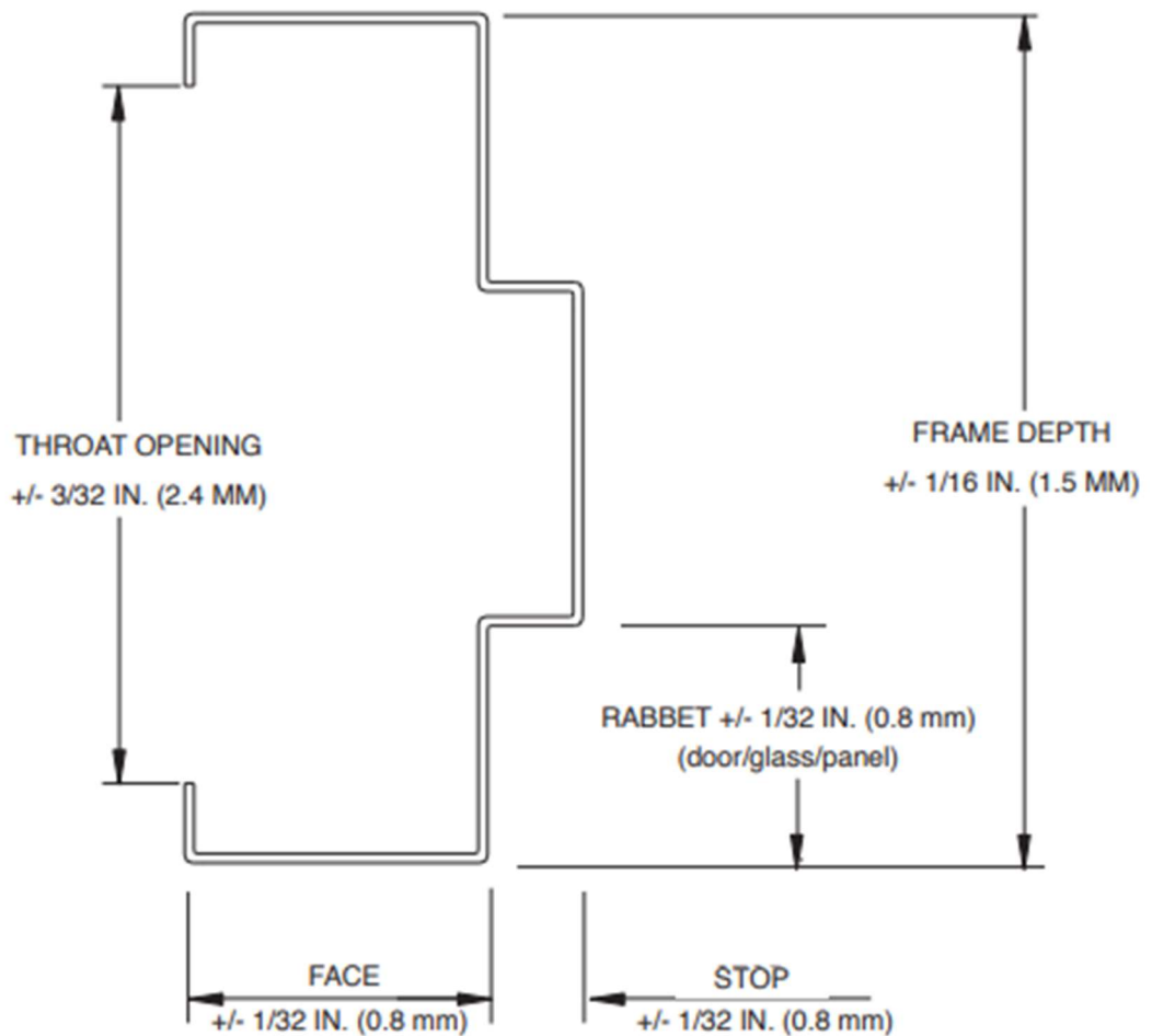
Figure 5 Section Profile Tolerances
