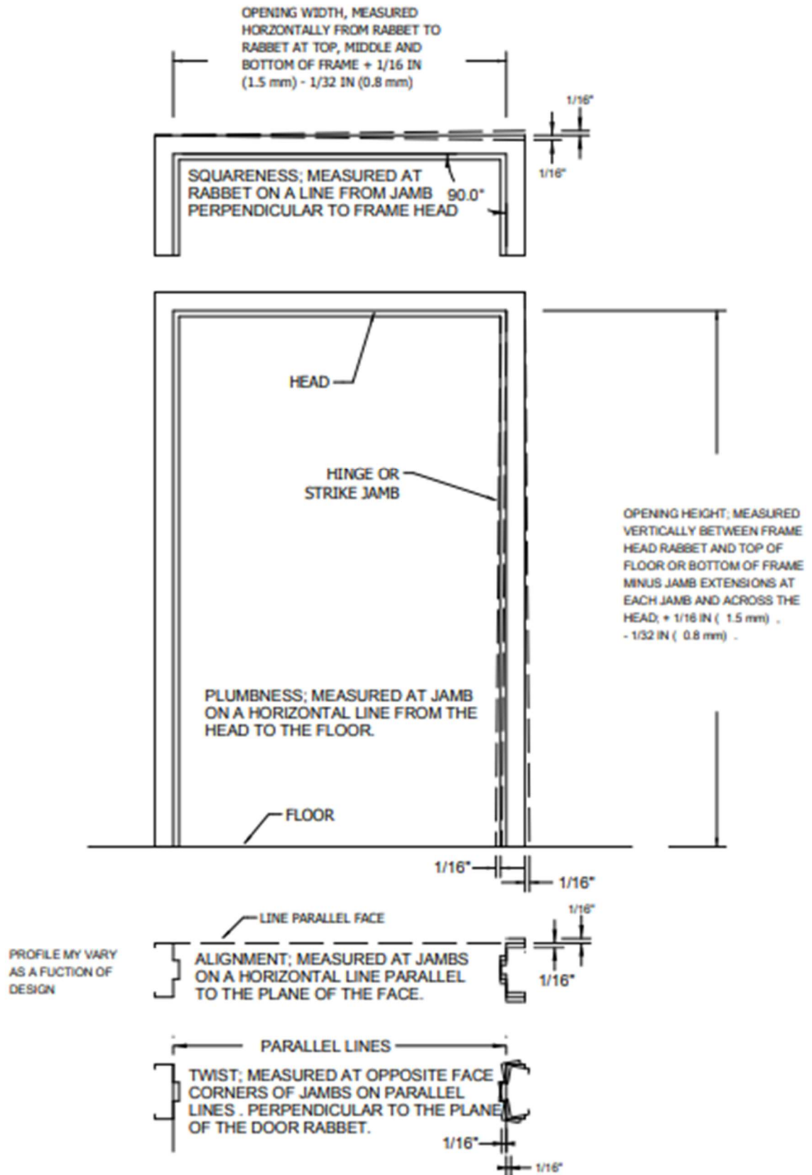
Figure 7 Installation Tolerances
