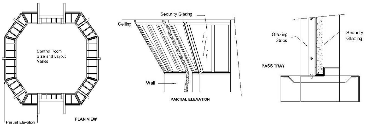
Figure 3 Typical Control Room Details
